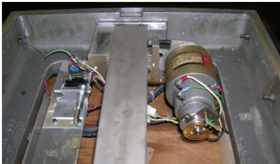
Close-up of Automec motor/encoder upgrade on an old S4 Autobend®
